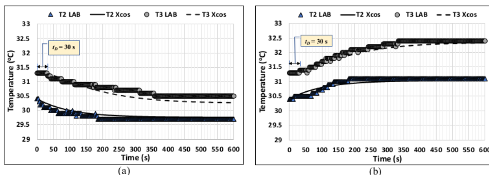
Figure 5. Open loop response to: (a) a step increase and (b) a step decrease, change in f(t) .
