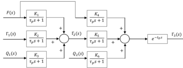
Figure 2. Block diagram of TTTS with dead time.
