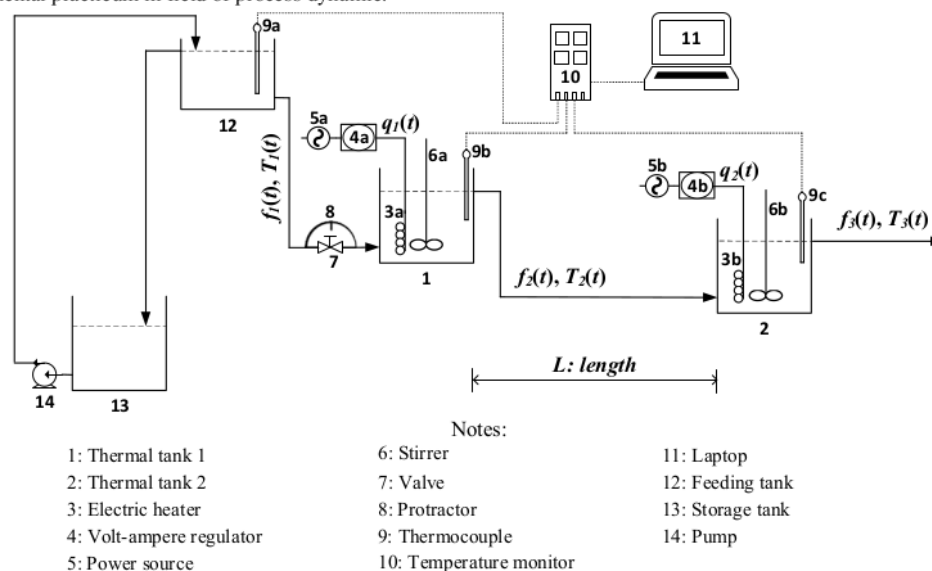
Figure 1. Experimental apparatus setup: two-thermal-tank-series.
