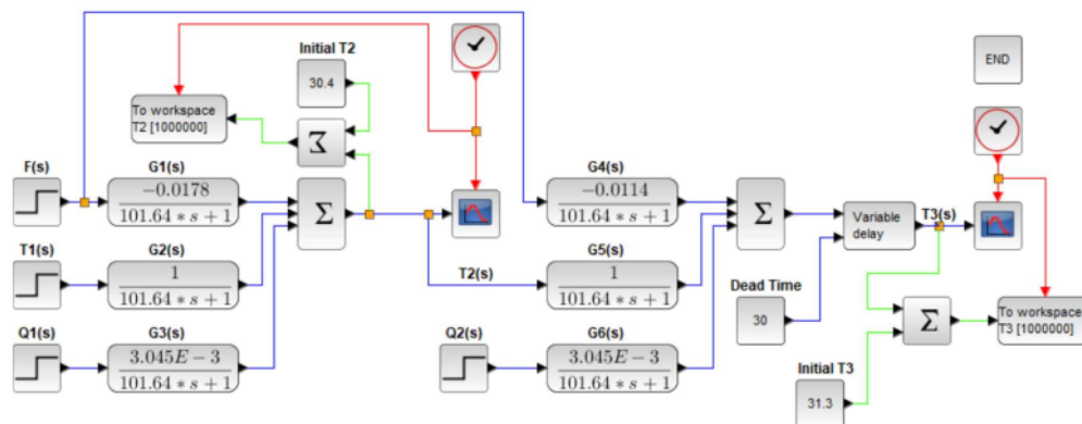
Figure 6. Xcos model of TTTS with dead time.
