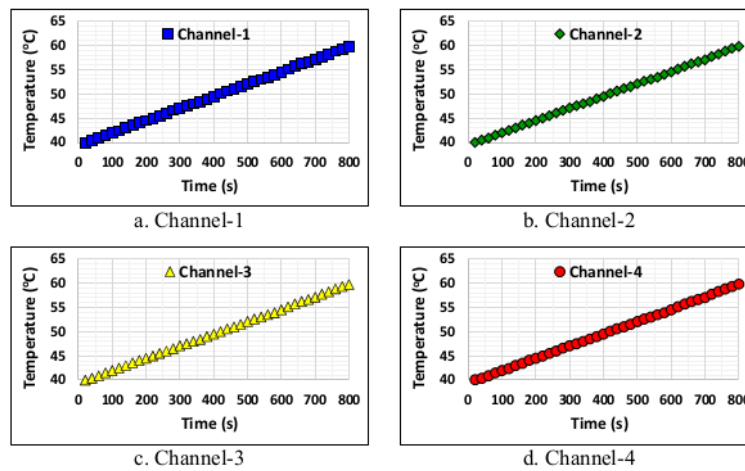
Figure 4. Performance of thermocouple 4 channels.
