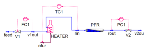
Figure 2. Model A in the control configuration of Heater-PFR-Series
