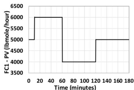
Figure 6. Set-point Changes in Controller FC1
