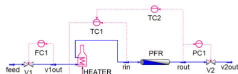
Figure 4. Model C in the control configuration of Heater-PFR-Series
