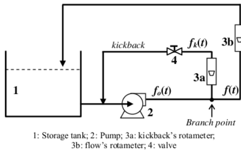
Figure 1. Open loop experimental apparatus setup.
