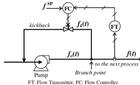
Figure 2. Proposed flow control configuration.
