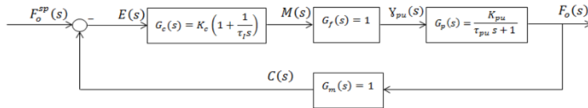
Gambar 3. Diagram blok loop tertutup.
