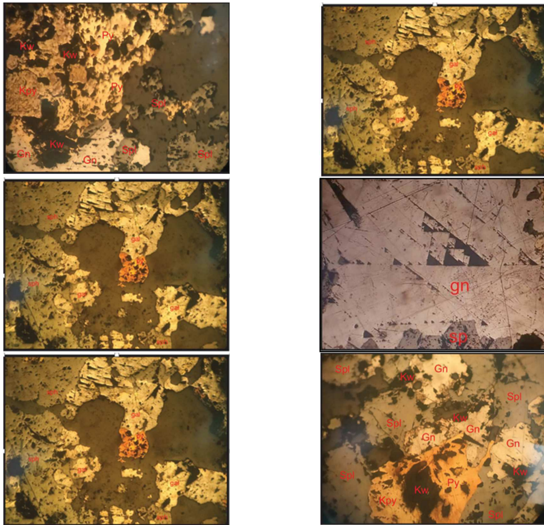
FIGURE 3. Sample shows Cp = Chalcopyrite, Gn = Galena and Sp = Sphalerite were growing together and crosscutting each other.
