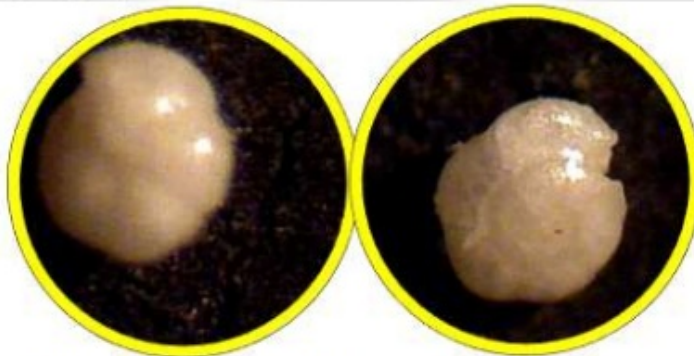
Clavulinoides indiscretus (210 ftm)
