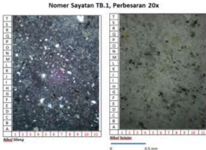
Gambar 3.1. Sayatan petrografi sampel 1-TB.1
