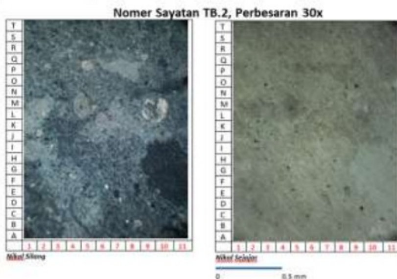
Gambar 3.2. Sayatan petrografi sampel 2-TB.2
