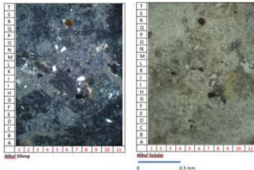
Gambar 3.8. Sayatan petrografi sampel 8-TB.6
