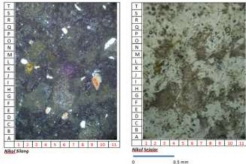
Gambar 3.3. Sayatan petrografi sampel 3-TB.3
