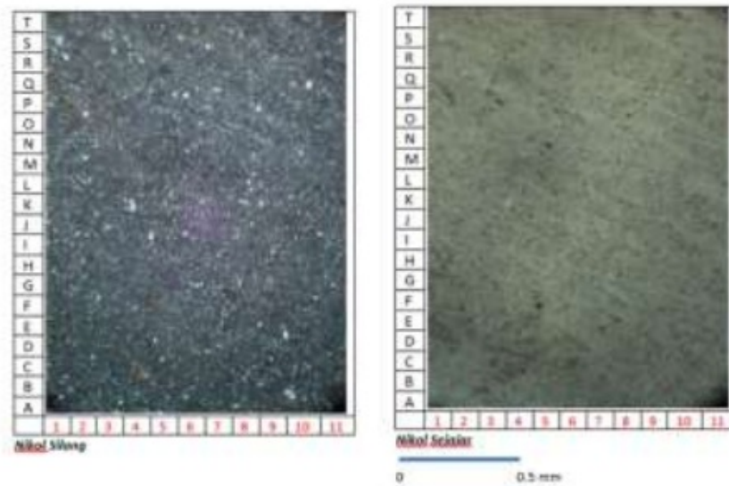
Gambar 3.5. Sayatan petrografi sampel 5-TB.4
