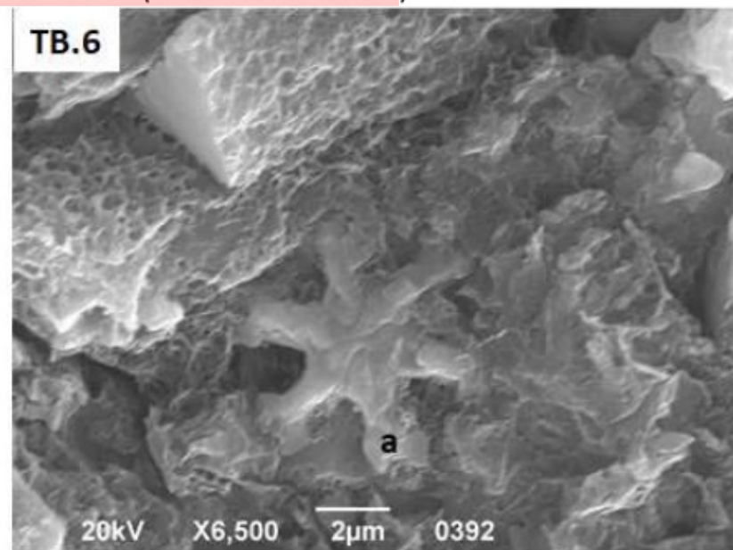
a) Discoaster deflandrei
