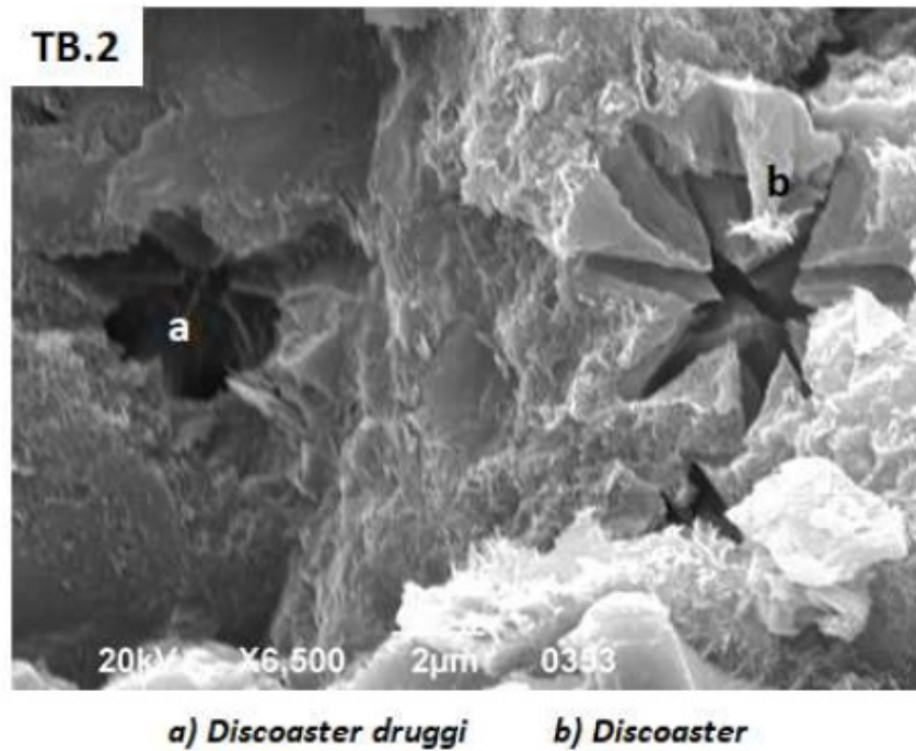
Gambar 5.15. Nanofosil Discoaster druggi dan Discoaster (?) (Sampel TB 2)
