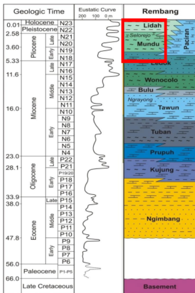
Figure 2. Regional stratigraphy [5].
