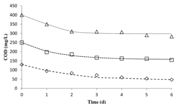
Fig. 3. COD consumption of B. braunii under different initial substrate from simulation of logarithmic model. 130 mg/L COD ( \diamond ), 250 mg/L COD ( \square ), 400 mg/L COD ( \Delta ); simulated result of 400 mg/L (.....), 250 mg/L COD (-----), 130 mg/L COD (— · —) logarithmic kinetic model.
