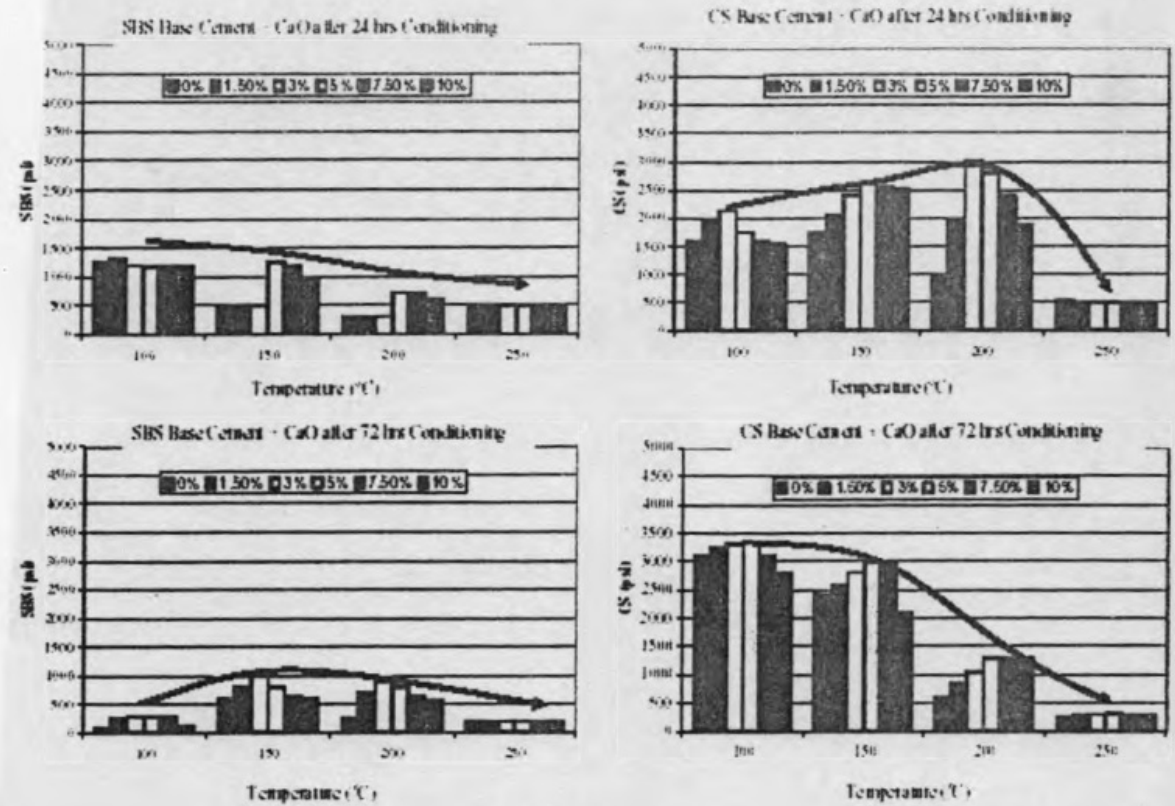
Figure 14 – The Effect of CaO addition on Base Cement.
