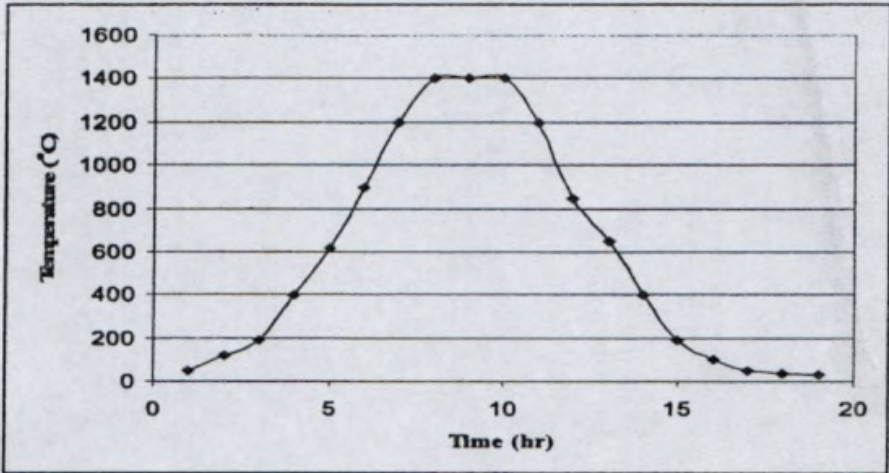
Figure 2 – CaO and MgO burning process.
