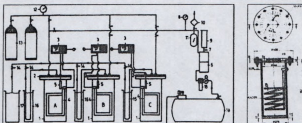
Figure 8 - Schematic Diagram of Modified Pressure Curing Chamber.
