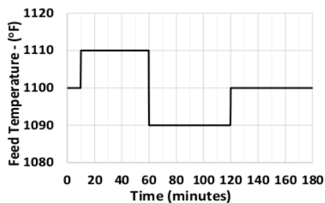
Figure 13. Disturbance Changes in Feed Temperature.
