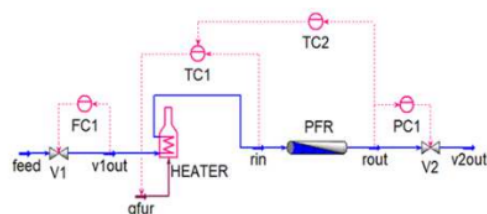
Figure 4. Model C in the control configuration of Heater-PFR-Series.
