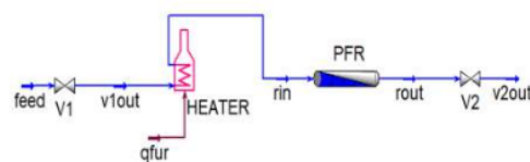
Figure 1. UniSim flowsheet of Heater-PFR-series.
