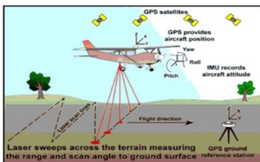
Figure 3. Working Principle of LiDAR (Nawangsidi, 2009)
