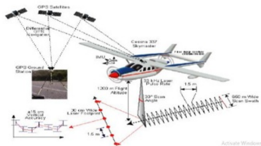
Figure 4. Representation of LiDAR Technology Data Acquisition (Putra, 2016)
