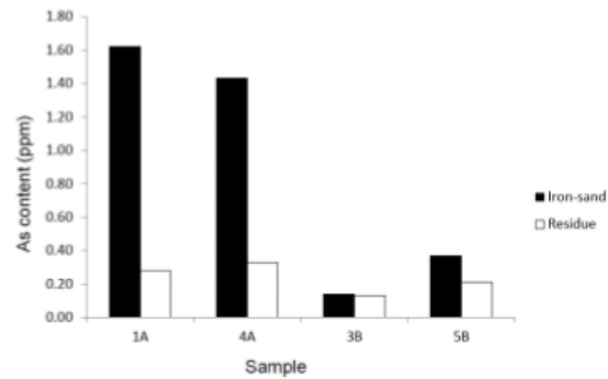
Figure 6: As content in the iron-sand and the residue
