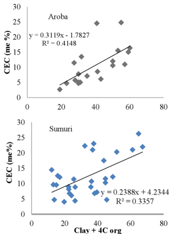
Figure-2: The relationship between CEC, clay, and organic C levels in Aroba and Sumuri Districts.
