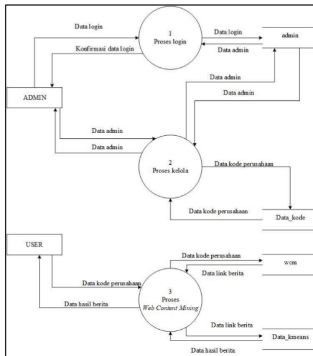
Gambar 3. DFD Level 1
