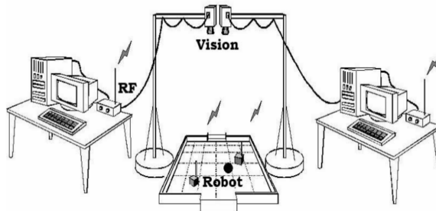
Gambar 1 Sistem Mirobot
