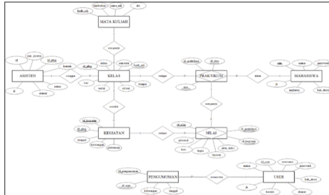
Gambar 5. Entity Relantionship Diagram (ERD)
