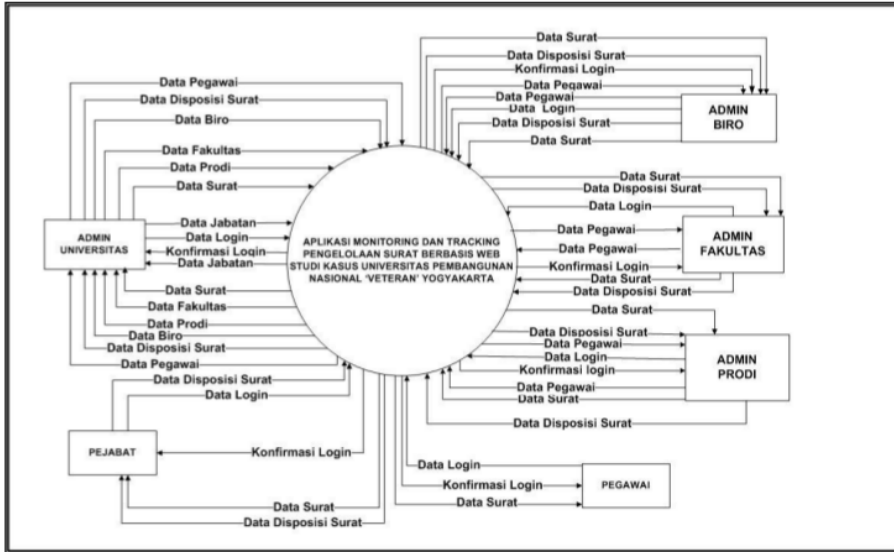
Gambar 1. DFD Level 0
