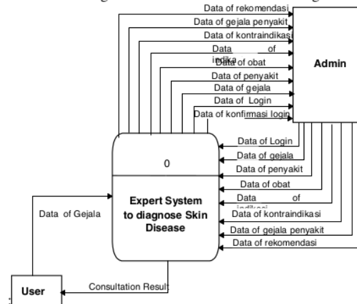
Figure 1 DFD level 0
