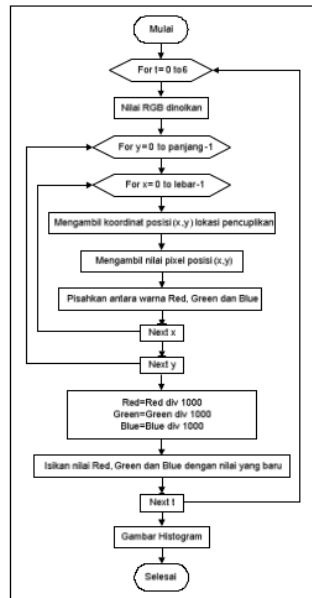
Gambar 4 Flowchart Histogram
