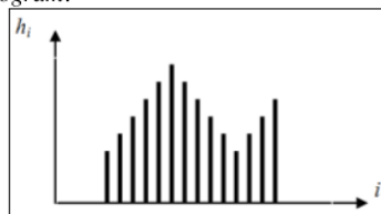
Gambar 2 Histogram Citra
