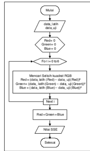
Gambar 5 Flowchart GetSSE
