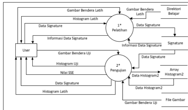
Gambar 3 Data Flow Diagram Level 1
