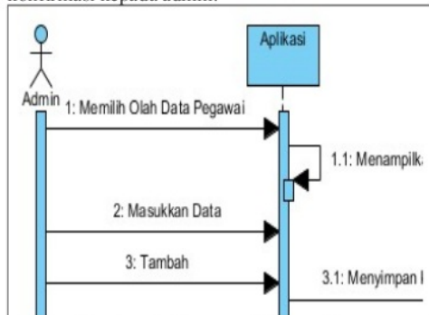
Gambar 6. Sequence Diagram Input
