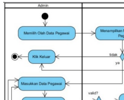
Gambar 4. Activity Diagram Input Data
