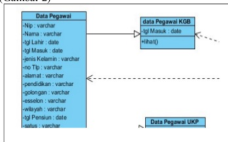
Gambar 2. Class Diagram
