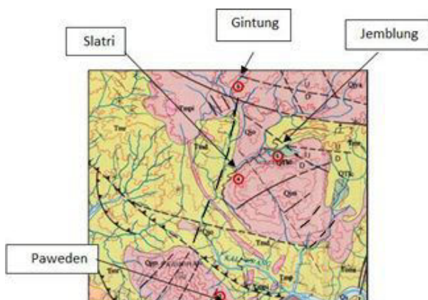
Figure 7. Locations of mass movements being analysed.
