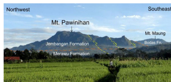
Figure 13. Step faulting and sliding of Mt. Pawinihan. Volcanic body that overstands on predominantly clay composing formation.
