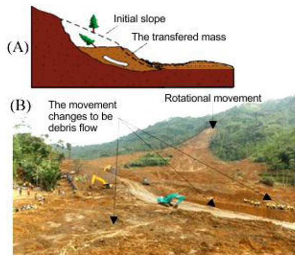
Figure 9. Analysis on Jemblung mass movement [15], modified.
