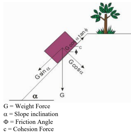
Figure 2. Stress distribution acting on a slope [9].
