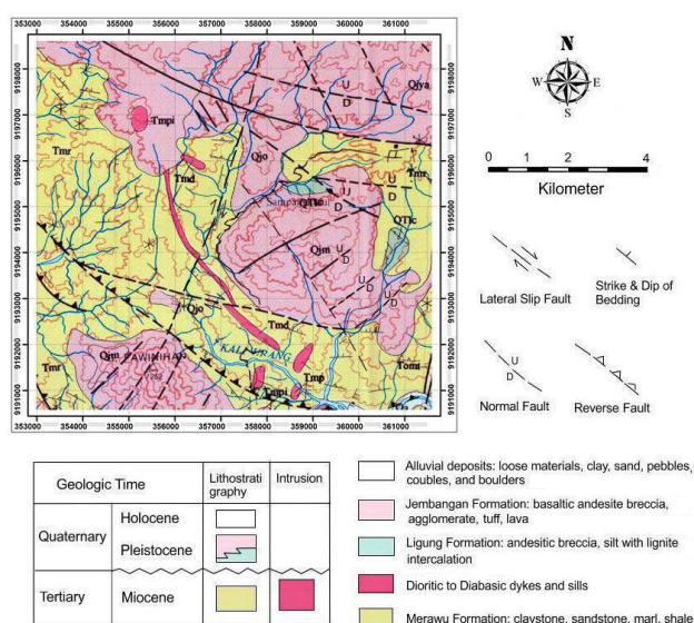
Figure 6. Geologic map of the Karangobar area.
