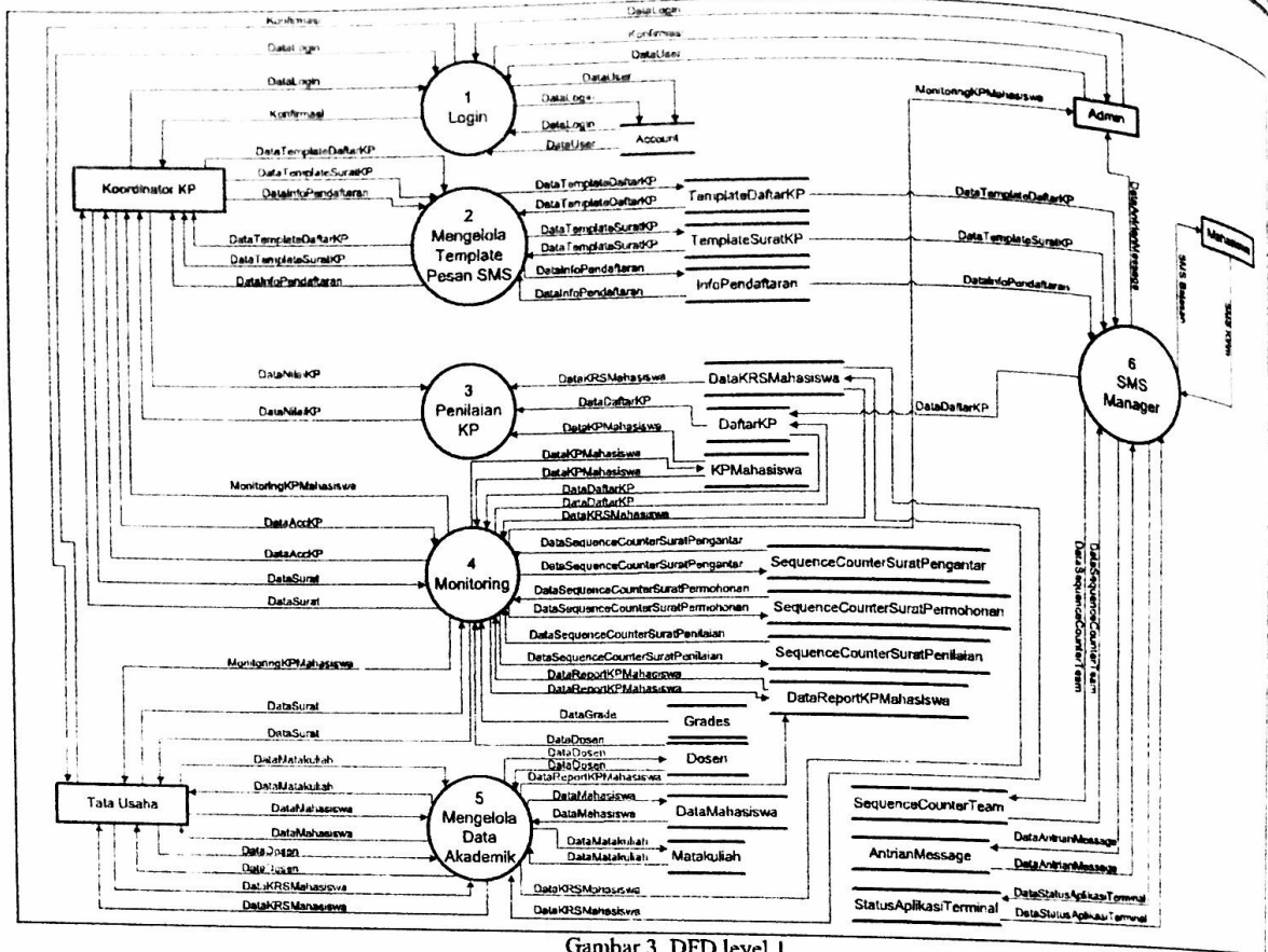
Gambar 3. DFD level 1
