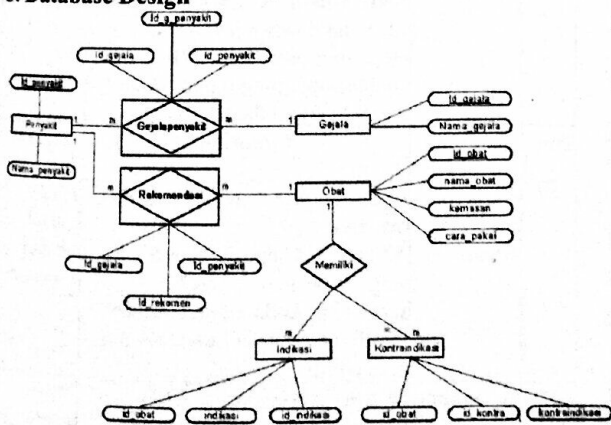
Figure 3 E-R Diagram
