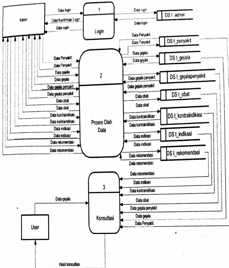
Figure 2 DFD Level 1
