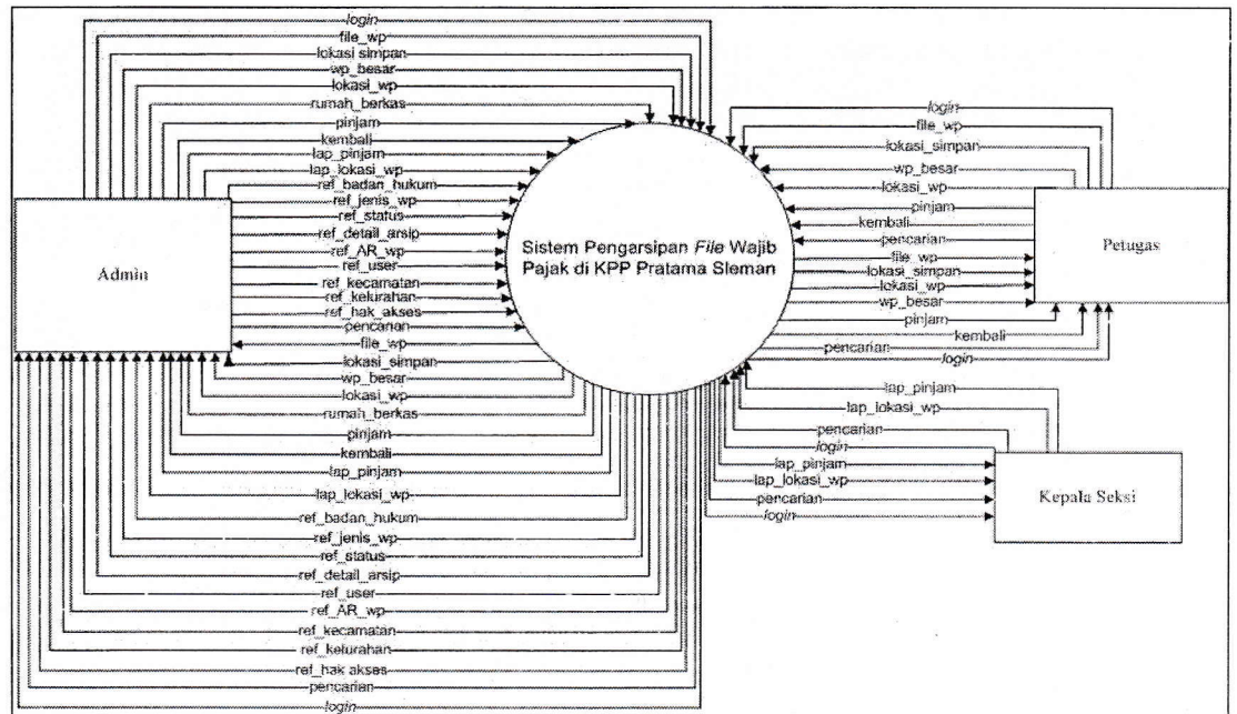
Gambar 1. DFD Level 0
