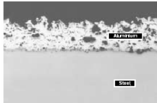
Figure 5: Thermal Spray Coating Factors Affecting Choice
