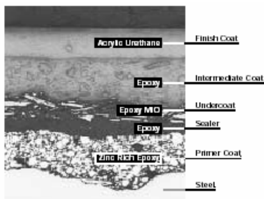
Figure 3: Protective Paint System Finishes
