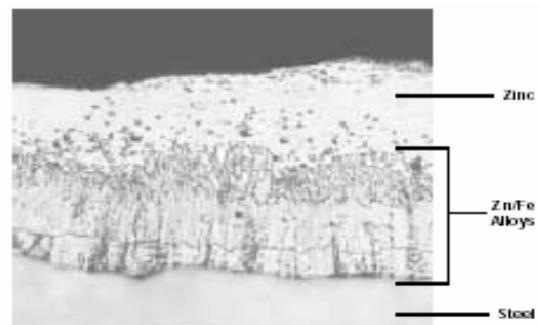
Figure 4: Hot-dip Galvanizing
