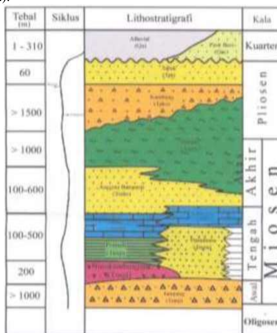
Figure 2. Regional Stratigrafi of Pangandaran (Simanjuntak and Surono, 1992)
