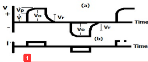
Fig. 2. (a) Time domain IP signal received showing measured parameters. (b) Current wave form : square-wave is generated low frequency.
