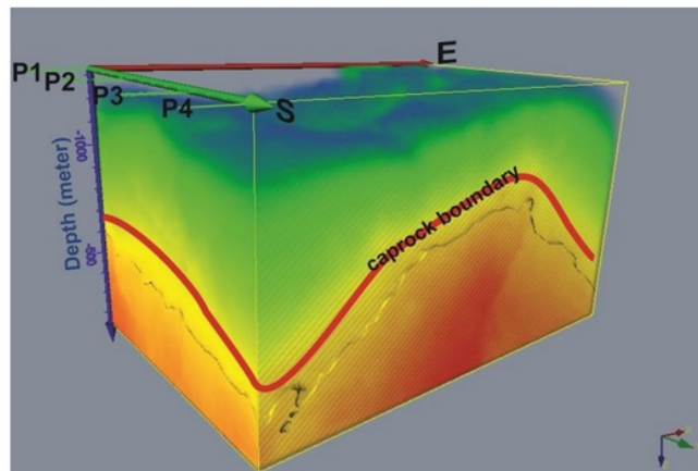
Figure 2. 3D Model of caprock in Candi Gedongsongo geothermal system.
