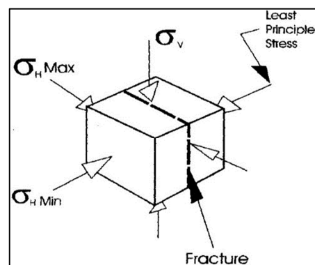
Figure 3. Main Stresses and Fracture Direction [9].
