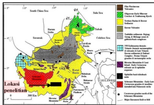
Gambar 2. Geologi Regional Kalimantan (Moss & Finch, 1997)
