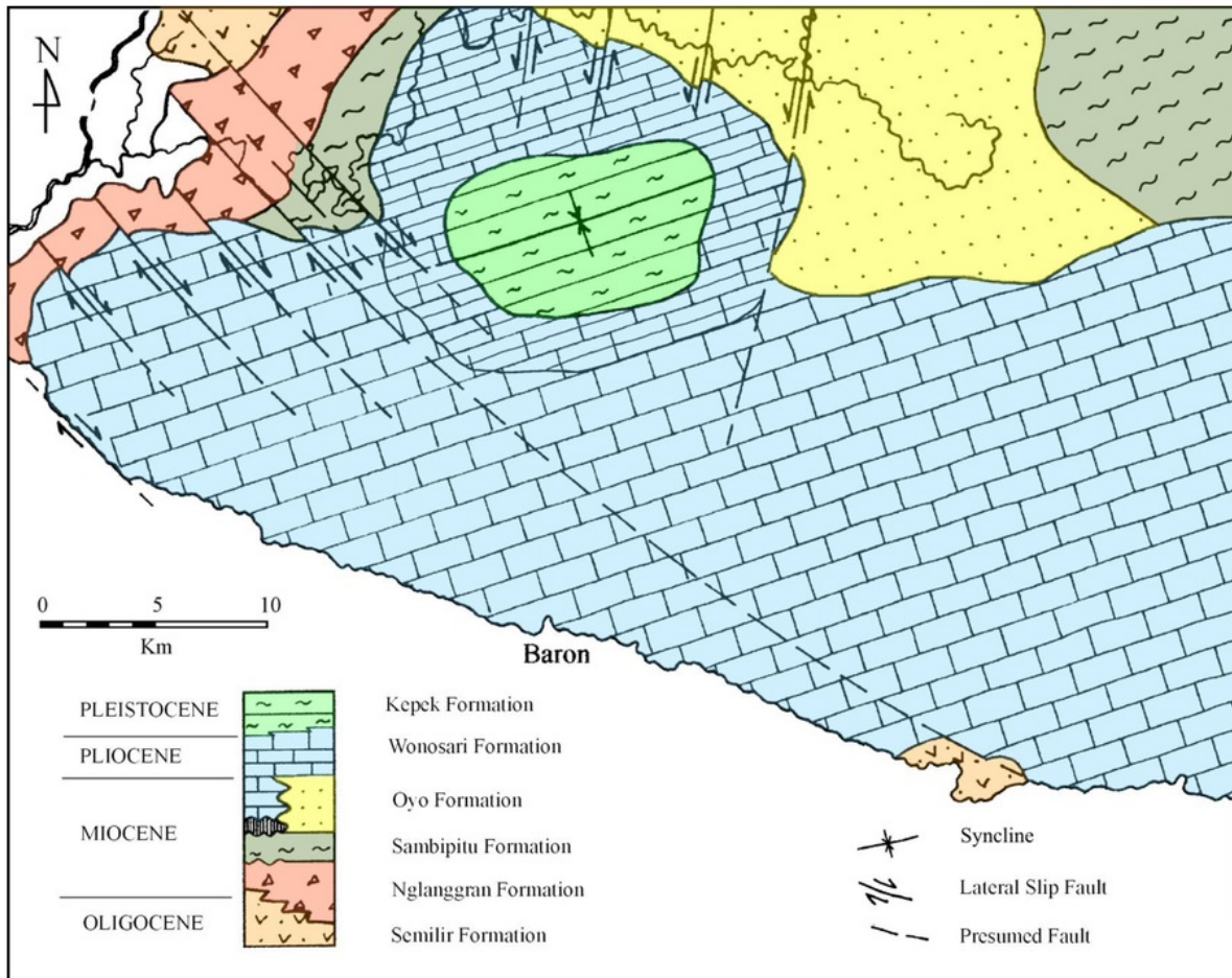
Fig 2. Geologic map of Gunungsewu area [10]
