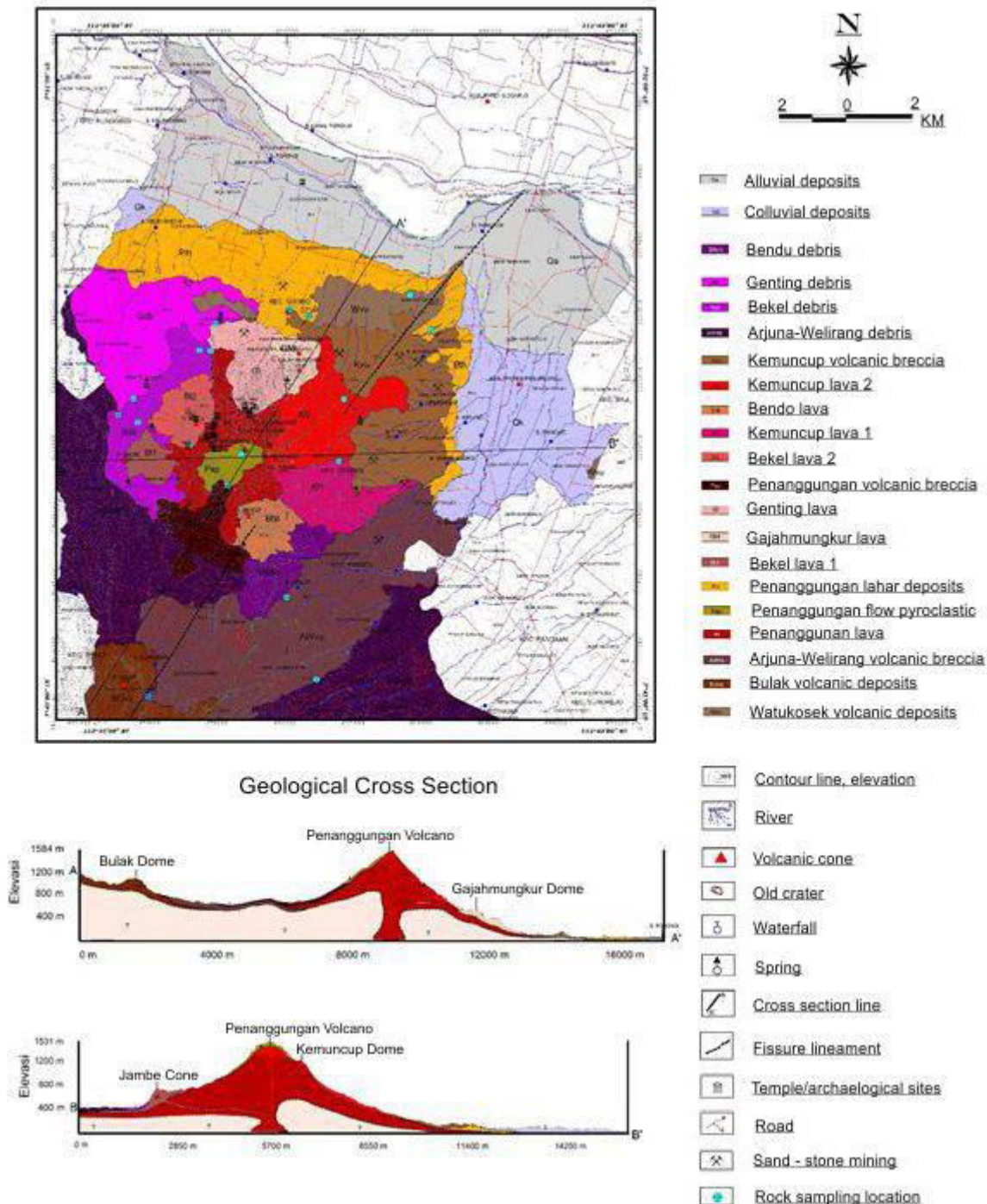
Figure 2. Geological map of Penanggungan Volcano and surrounding area
