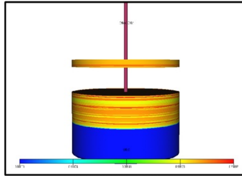
Figure 11- The Single Well Radial Model of Reservoir 'X'
