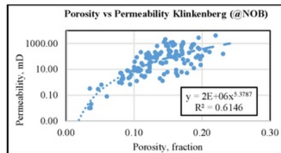
Figure 3- Conventional Transform Permeability
