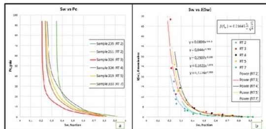
Figure 5- J-Function Curves Validate PGS Rock Types
