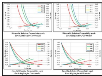
Figure 9- SCAL End Point Data for each Model
