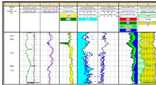
Figure 2- Corrected SCAL- Well-A Log Interpretation
