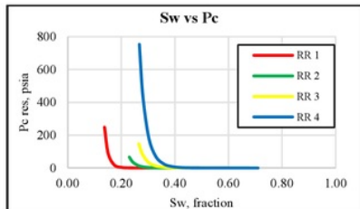
Figure 10- Capillary Pressure Data of Core-model to be used also for PGS-Model
