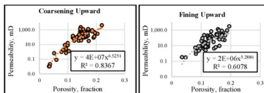
Figure 8- Conventional porosity-permeability plot
