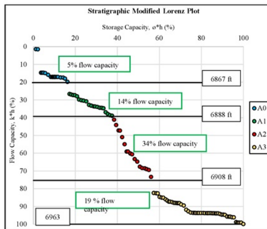
Figure 12- Flow zones based on stratigraphic modified Lorenz plot
