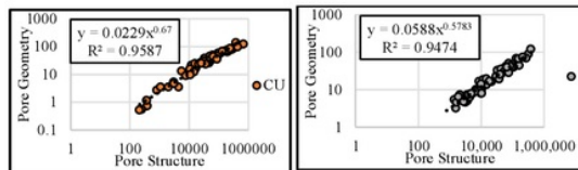
Figure 6- PGS plot based on the CU and FU petrophysical data, called RT 1 (CU) and RT 2 (FU)
