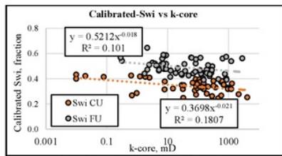
Figure 9- Calibrated-Swi for each rock type
