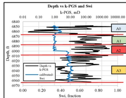
Figure 13- Swi and k-estimated (k-PGS) profile stratigraphically
