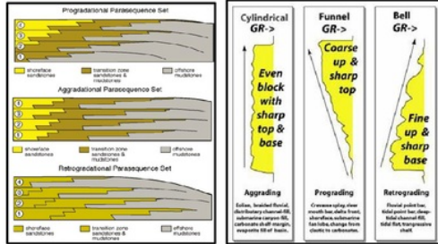
Figure 2- Parasequence set of formation and gamma ray log response
