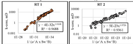
Figure 10- Permeability prediction equation as function of \alpha and Swi for each RT.
