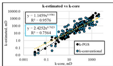
Figure 11- Estimated-permeability towards core permeability as validation
