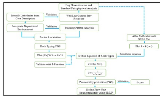
Figure 3- Workflow used based on core data and well log
