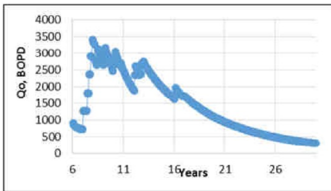
Figure 3. Performance Production Field Development Scenario "A"
