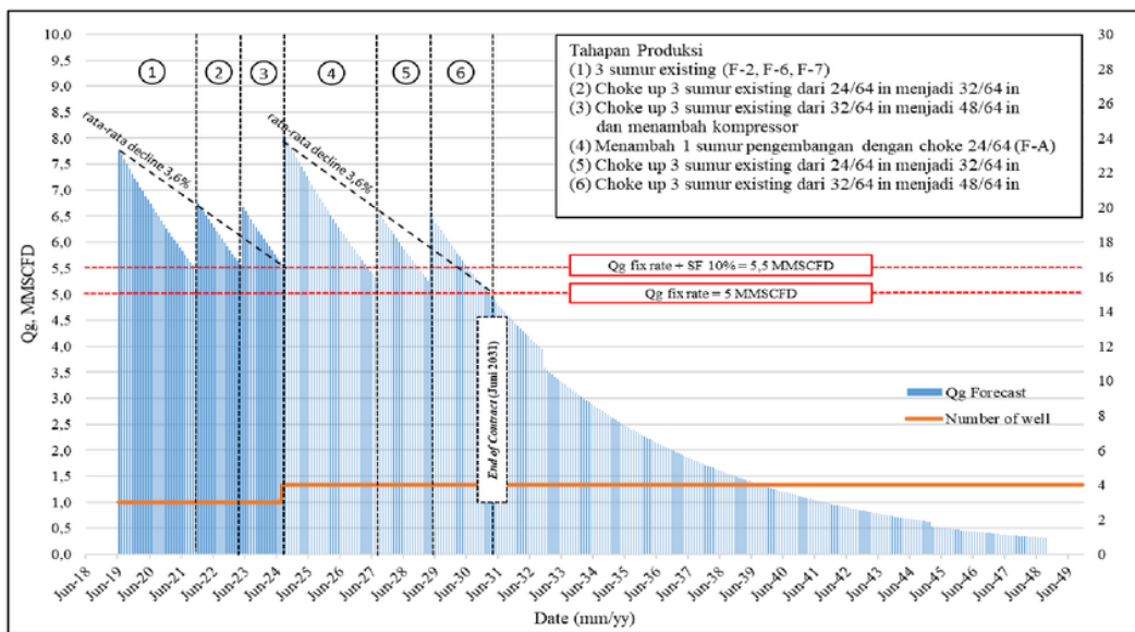
Figure 3. Gas Production Planning Pattern
