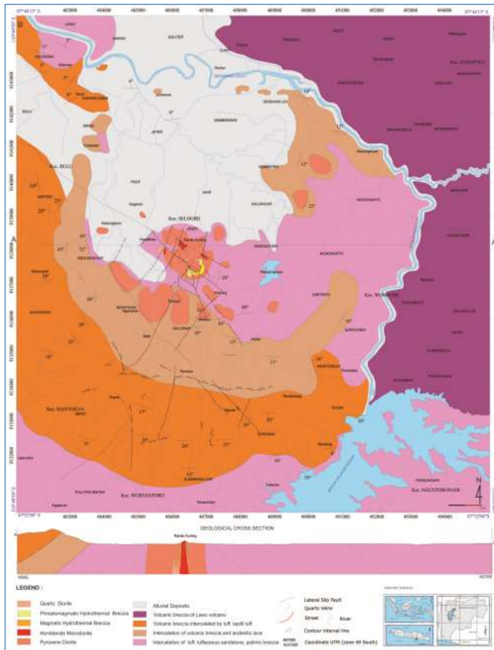
Fig.2. Geological Map of Selogiri area and its vicinity (Modified from Hartono, 2010 and Suasta and Sinugroho, 2011).
