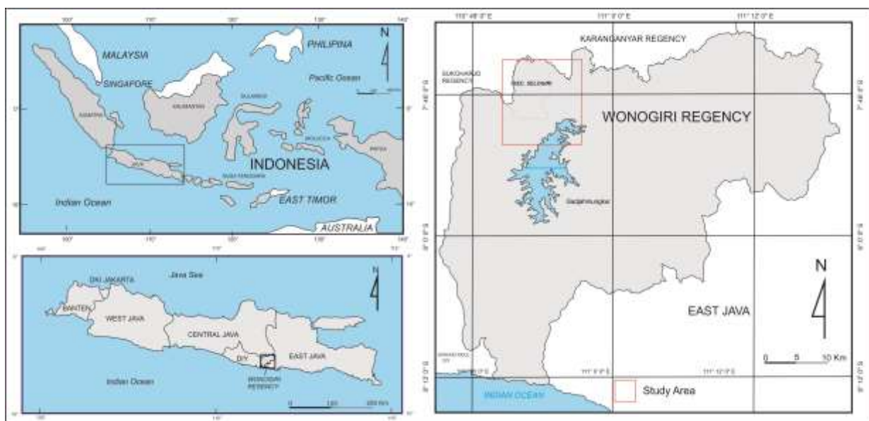
Fig.1. Location map of Selogiri area, Wonogiri
