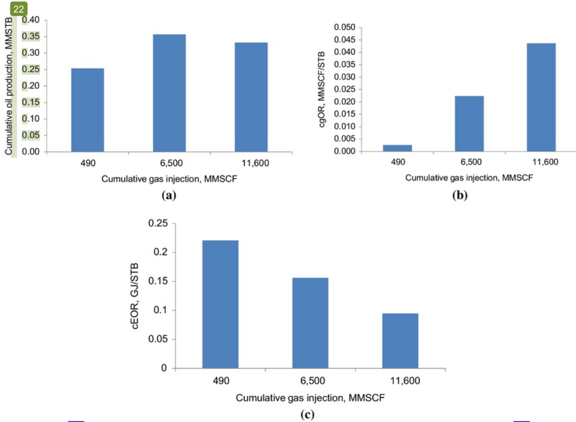
23 Figure 5. Effect of cumulative gas injection on cumulative oil production, cgOR and cEOR in CSS-gas top injection. (a) Cumulative gas injection vs. cumulative oil production, (b) Cumulative gas injection vs. cgOR, (c) Cumulative gas Injection vs. cumulative energy oil ratio (cEOR).
