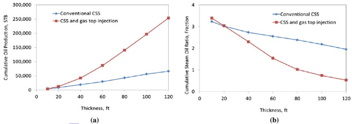
35 Figure 6. The comparison of cumulative oil production and CSOR on the both of methods. (a) Cumulative oil Production vs. thickness, (b) CSOR vs. thickness.
