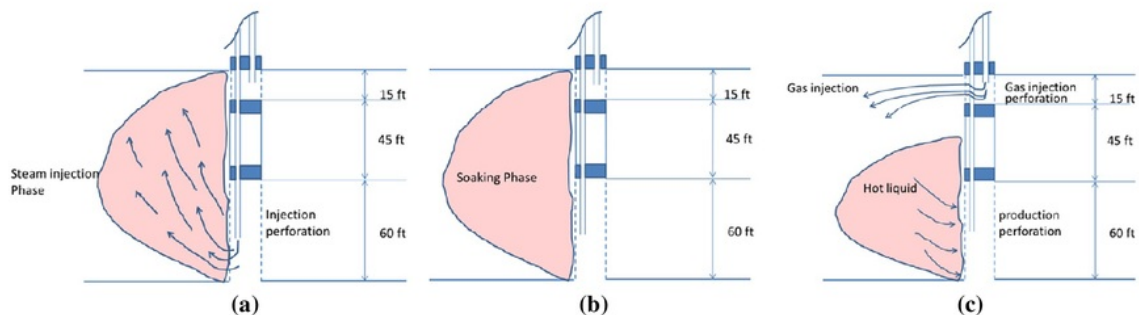
Figure 1. Completion modified for CSS-gas top injection. (a) The steam injection period, (b) Soaking time period, (c) The CCS-gas top injection period.
