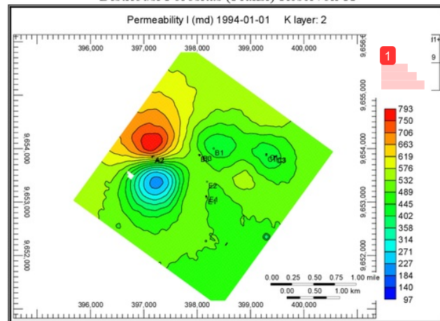
Gambar 6. Distribusi Permeabilitas Reservoir X
