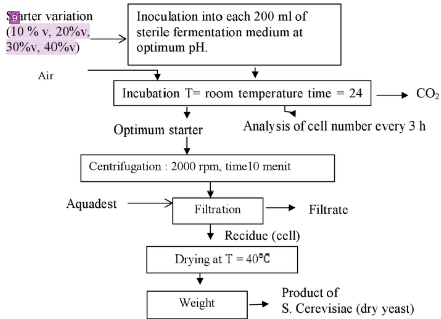
Figure 2. Flow diagram of fermentation and product separation of S. Cerevisiae .
