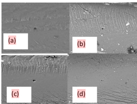
Fig. 2. Mophology of the: (a) pure Nafion, (b) the composite with the R = 0.05 (w/w), (c) R = 0.1 (w/w) and (d) R = 0.25 (w/w).
