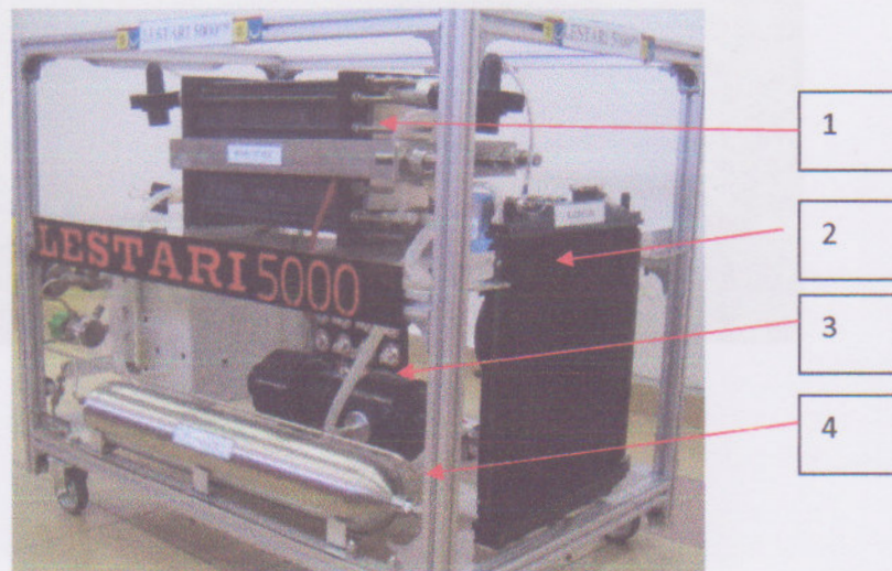
Figure. Exterior LESTARI 5000™ Power Generator System,(1) PEMFC, (2) HE,(3)Compressor, (4) Storage Hydrogen
