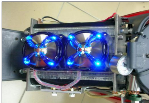
Open Air Cathode Fuel Cell Stack
