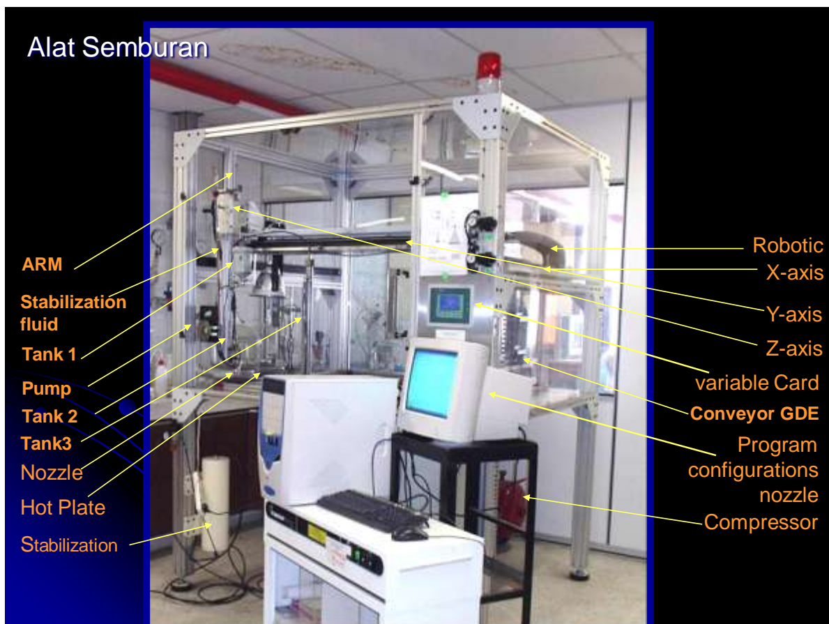
Figure. Robotic Spraying Machine
