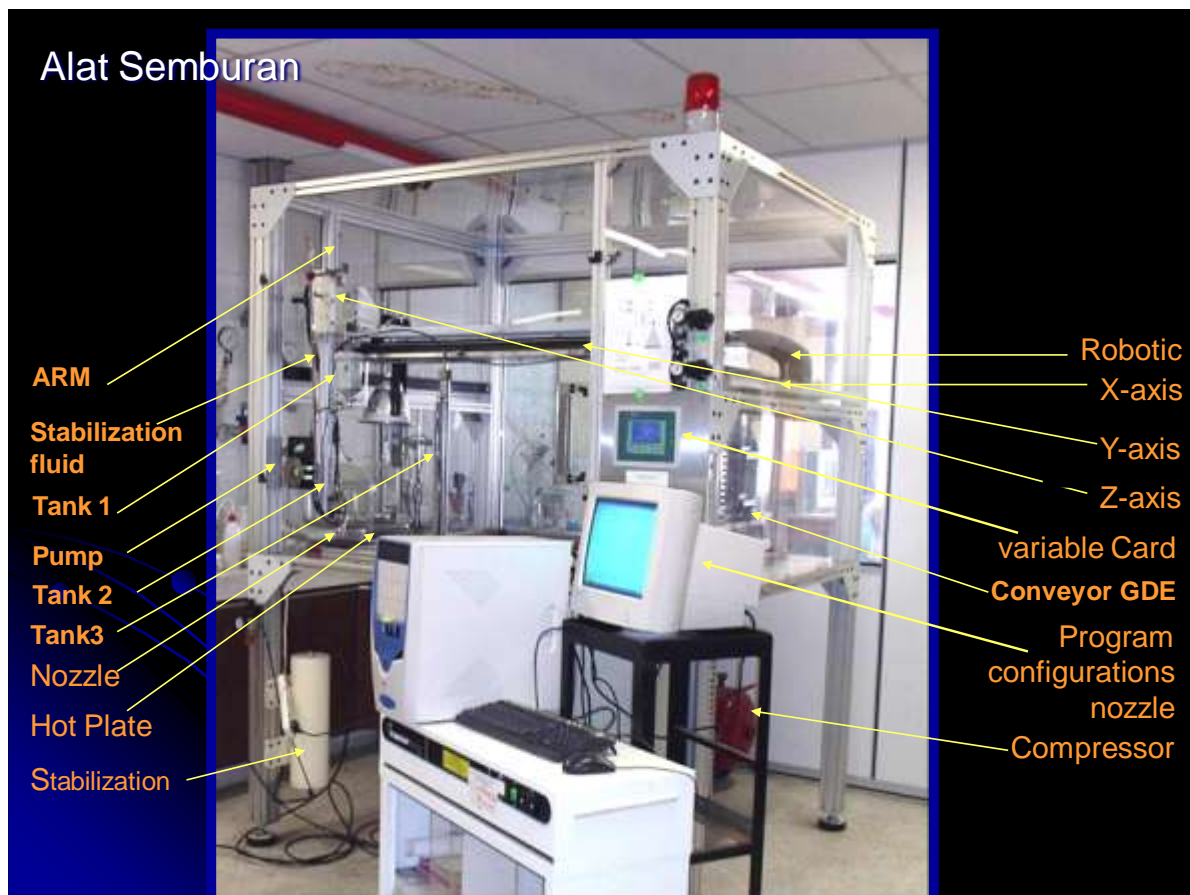
Figure 2. Teknologi Product of Robotic Spraying Machine
