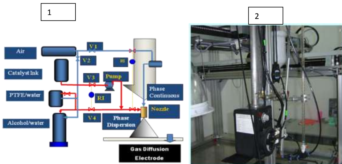
Figure 1. (1) Flow diagram of fluid and robotic spraying machine, (2) The X-Y spraying arm of the Robotic Spraying Machine
