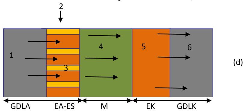
Figure 1. Design of Anode: (1). The anode part diffusion layer (GDLA), (2). The anode gas diffusion layer (EA), (3). Electrode support layer (ES), (4) Membrane layer (M), (5). Layers of electrode cathode (EK), (6) .gas diffusion layer (GDLK)
