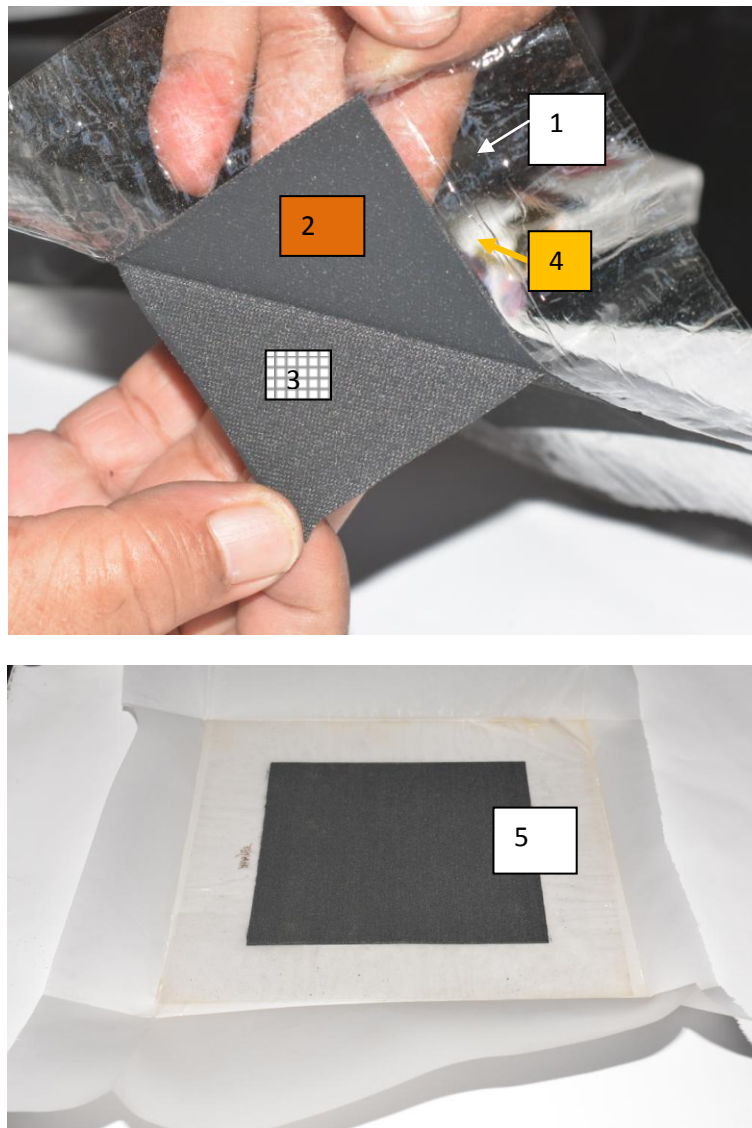
Figure MEA: (1) Membrane Nafion 117, (2) Anode, (3) GDLA, (4) electrode backers, (5) MEA
