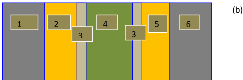
Figure 4. Configuration GDLA-EA-M-EK-GDLKE, commercial. (1) Gas diffusion layer (GDLA), (2). Electrode anode layer (EA), (3). Nafion Layer (N), (4) Membrane (M), (5). Electrode cathode layer (EK), (6). Gas diffusion Layer (GDLK)
