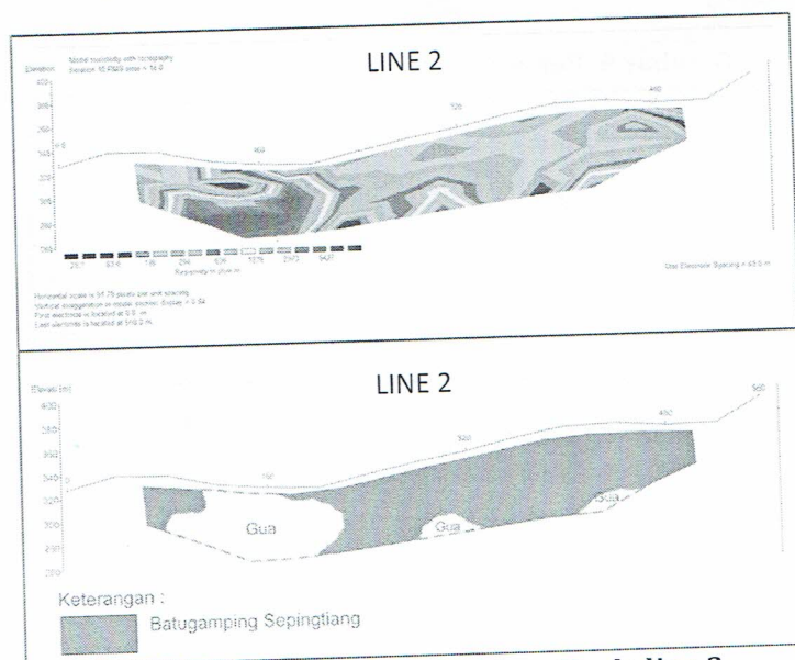
Gambar 5. Penampang dipole - dipole line 2
