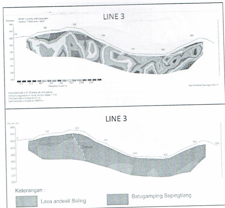
Gambar 6. Penampang Dipole - Dipole Line 3
