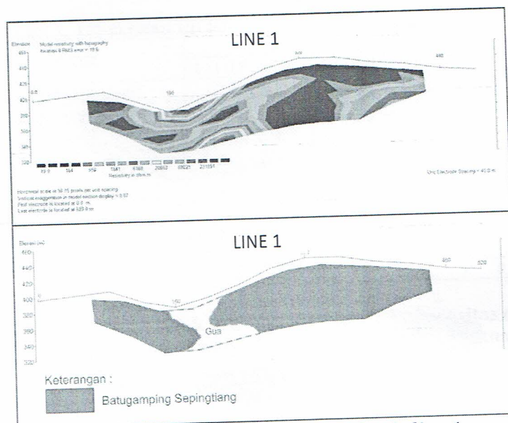
Gambar 4. Penampang dipole - dipole line 1
