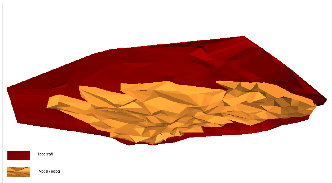
Gambar 3. Model geologi 3D endapan nikel
