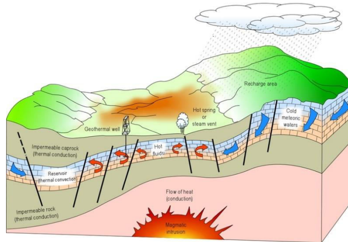
Figure 8. Geothermal system model ( http://www.indotoplist.com/info )
