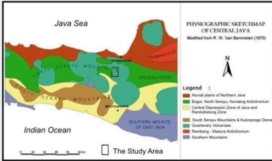
Figure 2. The Physiographic map of Central Java (Van Bemmelen, 1949)
